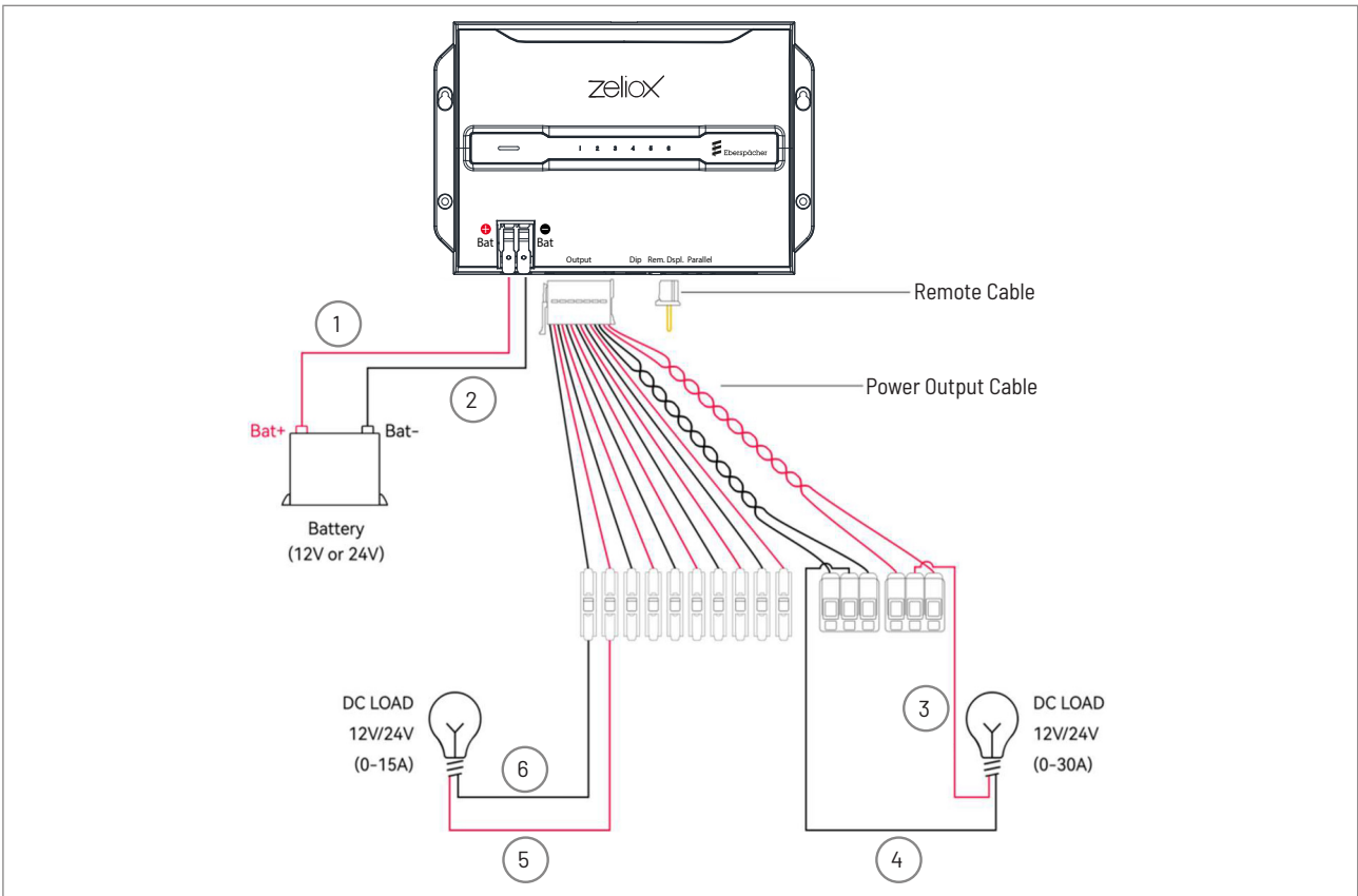
Figure 3: Single wiring
