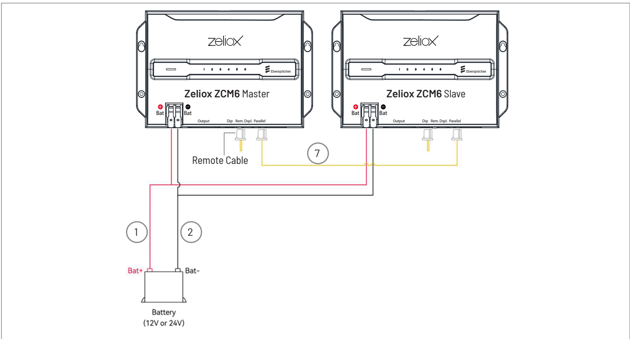
Figure 4: Parallel wiring
